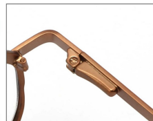
REPAIRABLE SPRING HINGE
